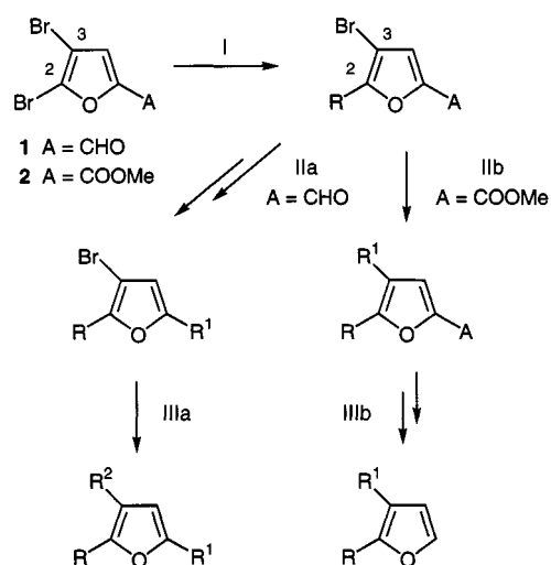
Scheme 1. General strategy for preparation of 2,3,5-tri- and 2,3-disubstituted furans from the 2,3-dibromofurans 1 and 2
