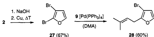
Scheme 4. Preparation [16b] and regioselective Stille reaction of 2,3-dibromofuran ( 27 )
