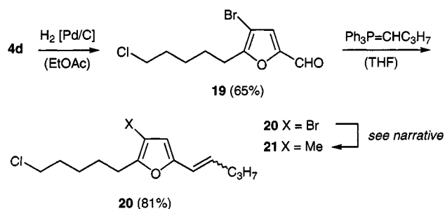
Scheme 2. Preparation of furan 20 from the 2-alkynylfuran 4d and attempted coupling reactions
