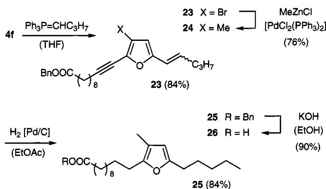
Scheme 3. The synthesis of the F_5 furan fatty acid ( 26 ) starting from the product 4f of the regioselective cross coupling at C-2
